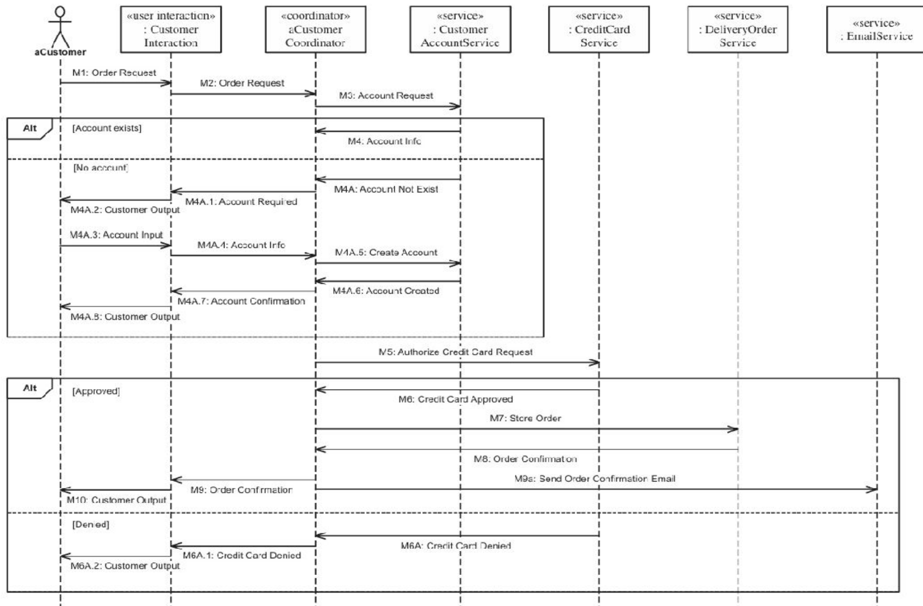
Figure 9.10. Generic sequence diagram for the Make Order Request use case: main and alternative sequences
