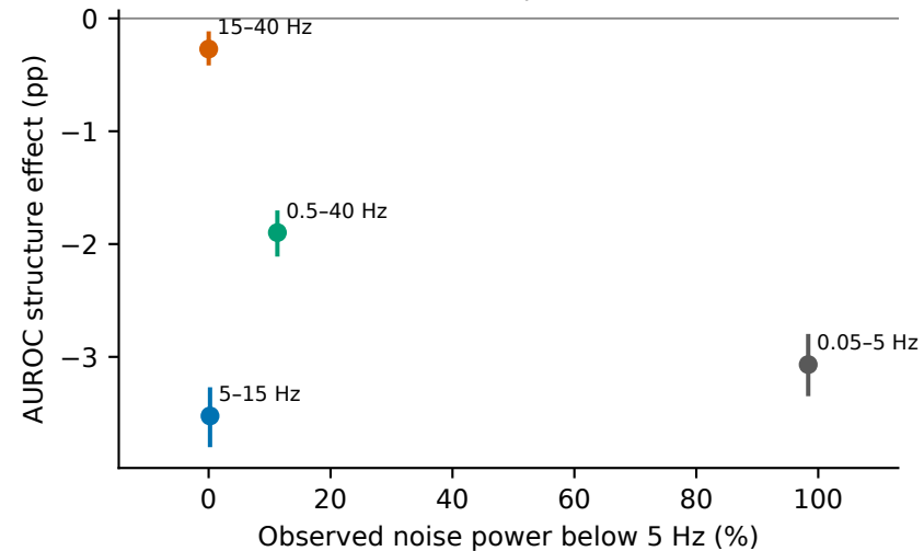
ResNet | 0 dB
