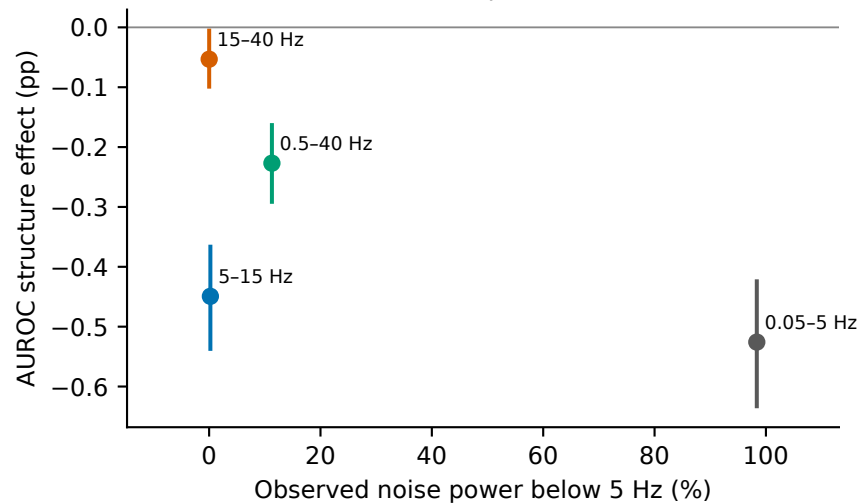
ResNet | 10 dB
