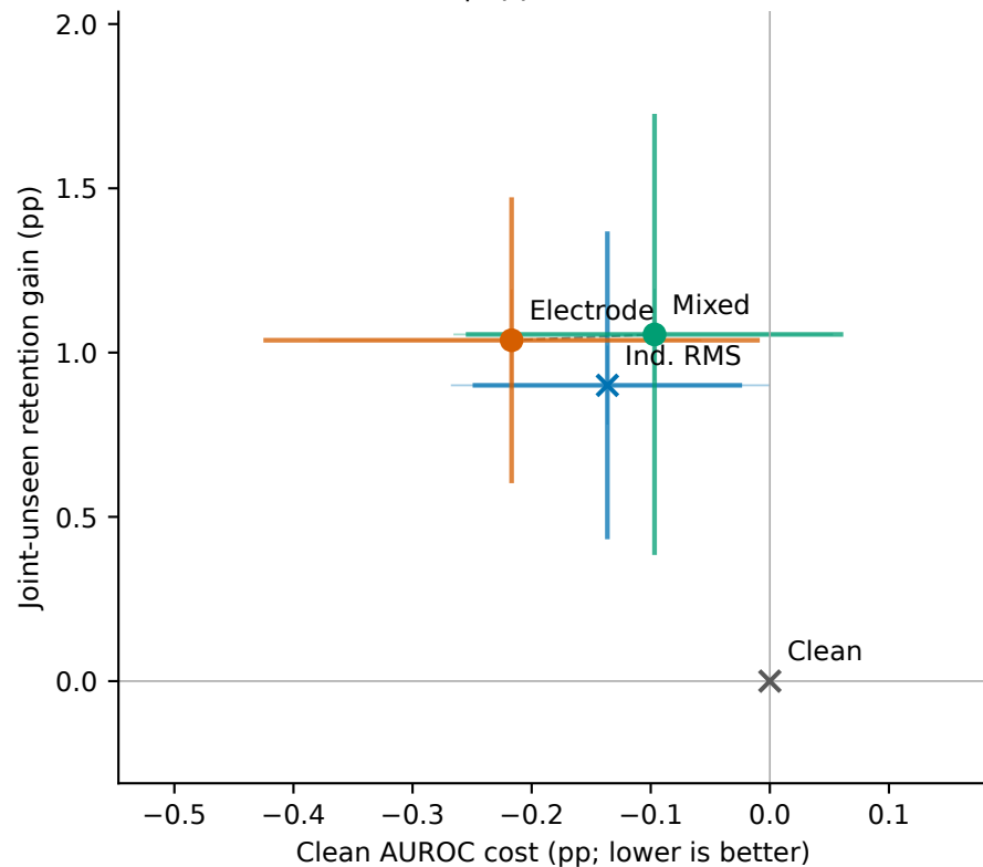
ResNet | upper-left is better
