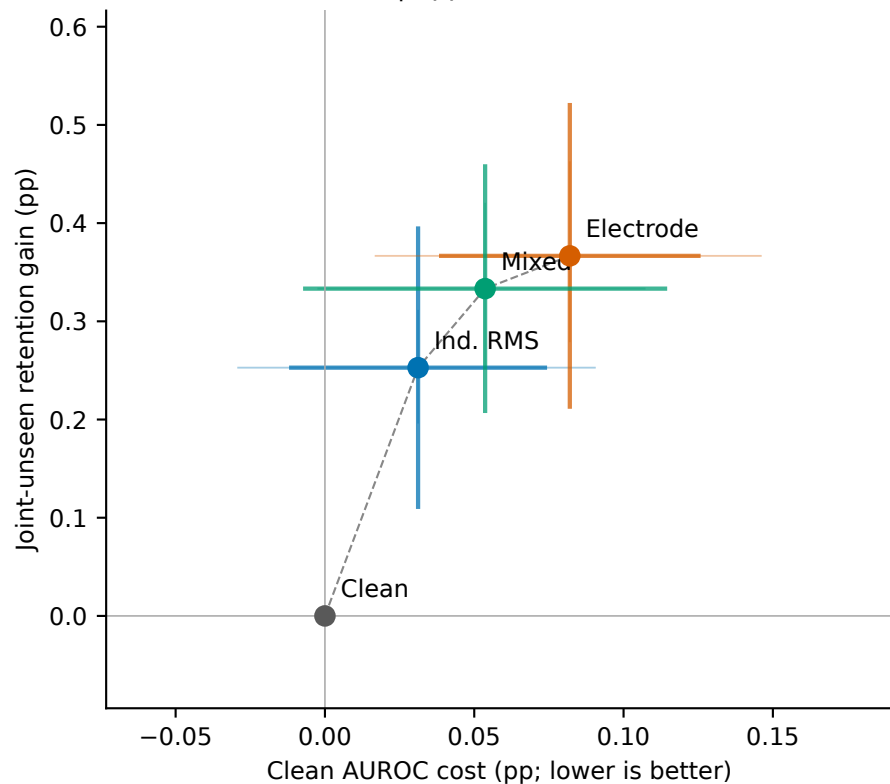
TCN | upper-left is better
