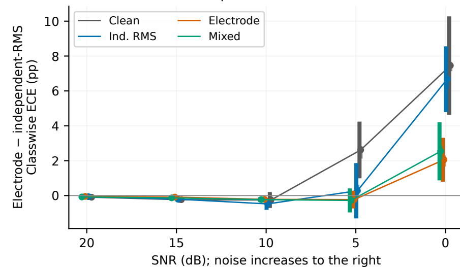
TCN | Phase 2: 5 seeds
