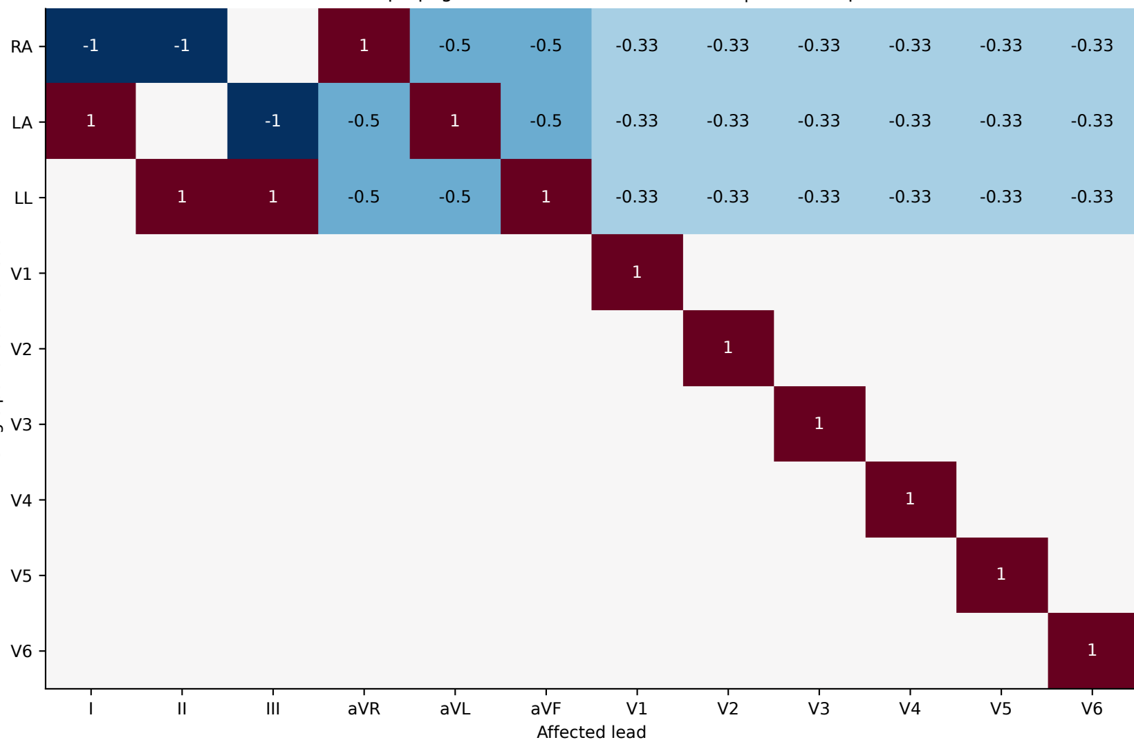
Unit-electrode propagation: A times each unit vector | 100 Hz experiment
