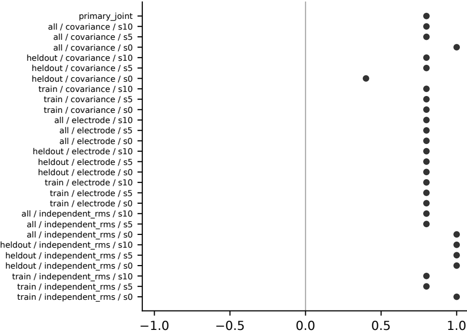
TCN | Spearman
