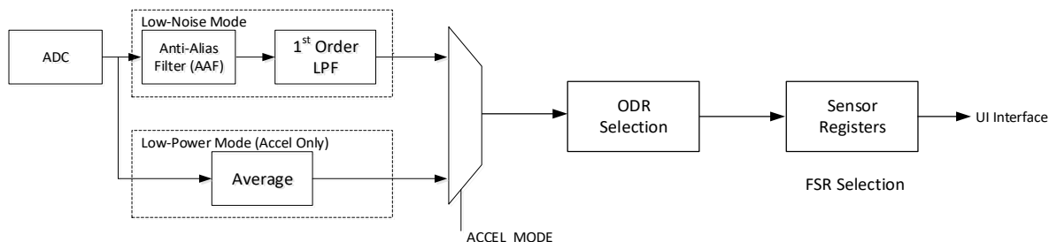
Figure 8. ICM-42670-P Signal Path
