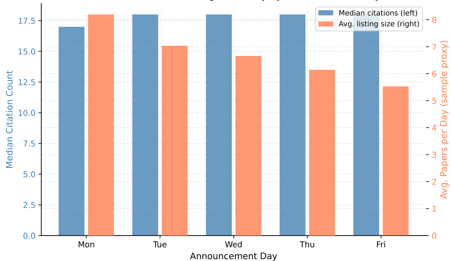
AandA: Citations vs Listing Size Proxy by Announcement Day
