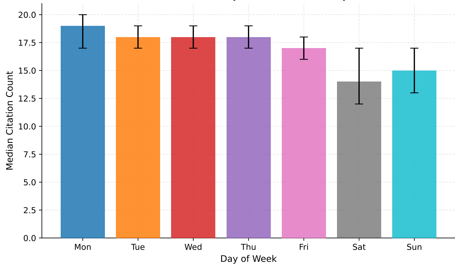
AandA: Median Citations by arXiv Submission Day (95% CI)
