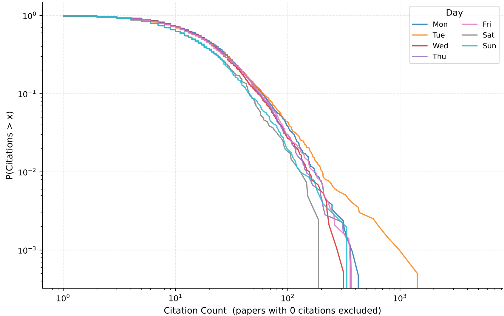
ApJ: Citation Distribution by Submission Day
