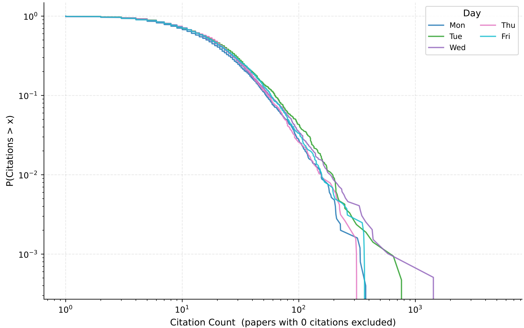
ApJ: Citation Distribution by Announcement Day
