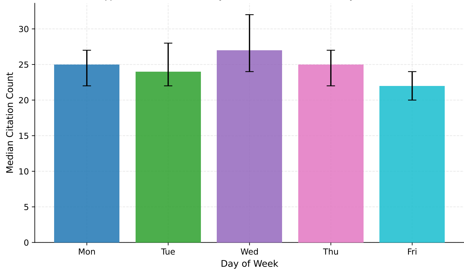
ApJL: Median Citations by arXiv Announcement Day (95% CI)
