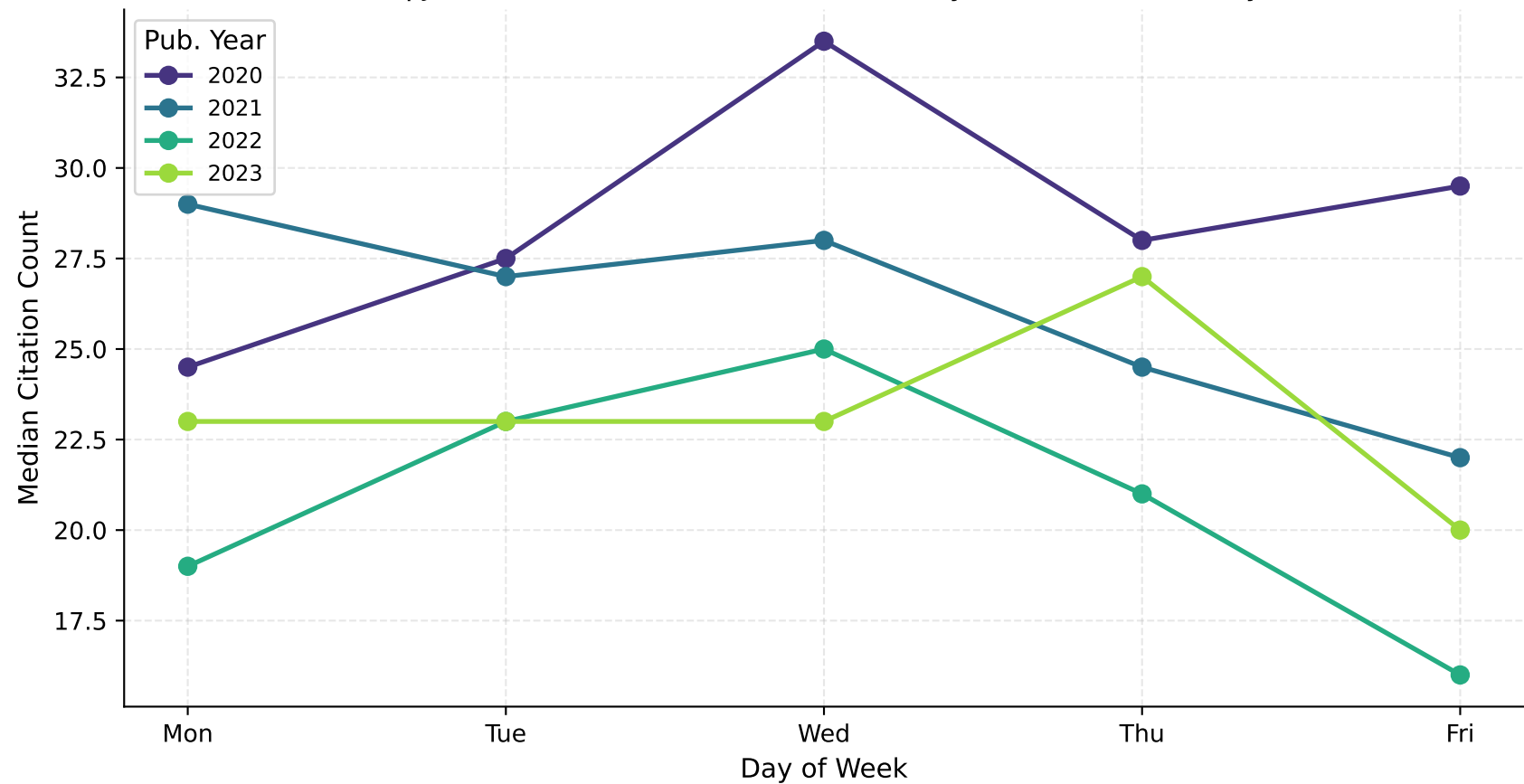
ApJL: Year-Stratified Median Citations by Announcement Day
