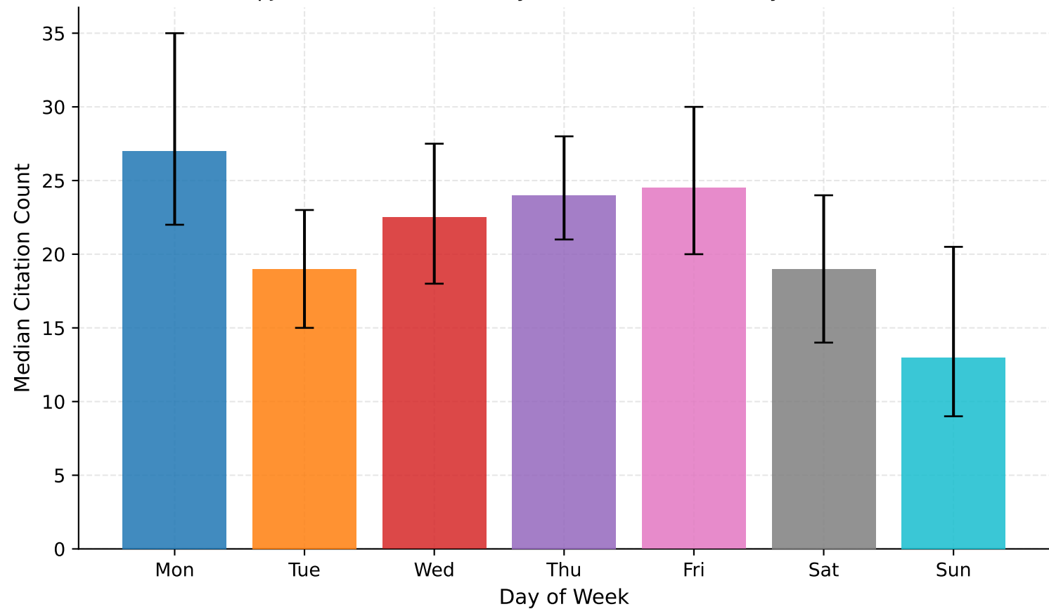
ApJS: Median Citations by arXiv Submission Day (95% CI)
