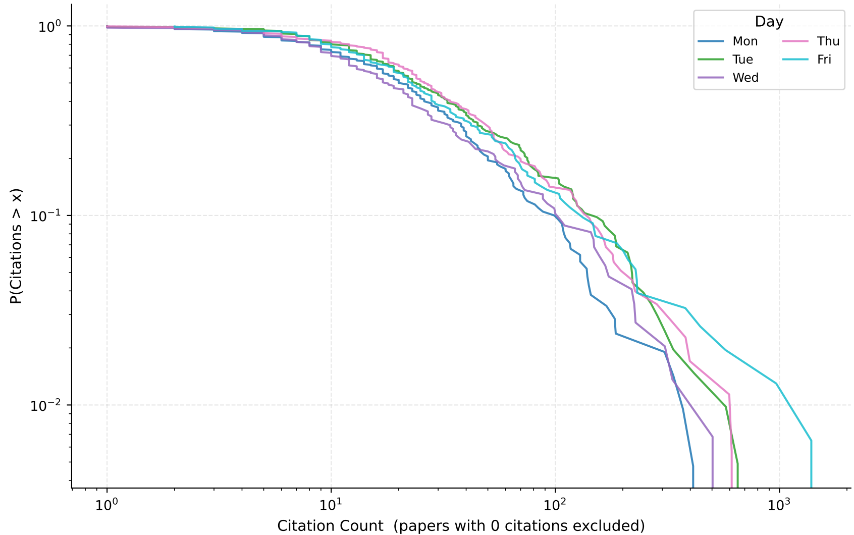
ApJS: Citation Distribution by Announcement Day
