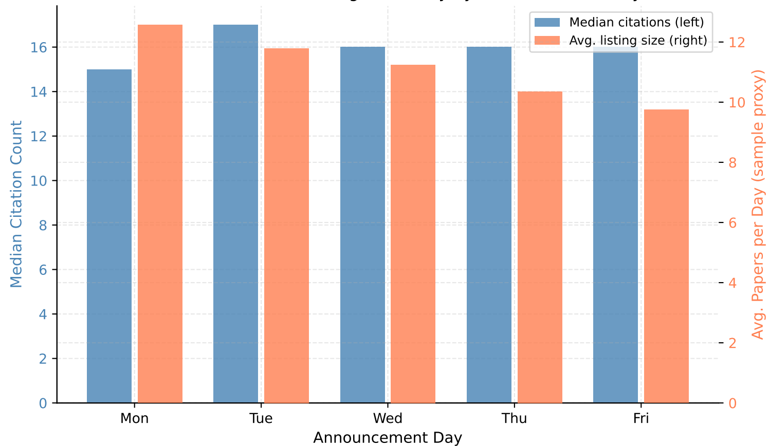
MNRAS: Citations vs Listing Size Proxy by Announcement Day
