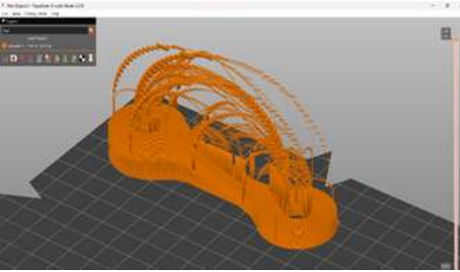
Fig. no:3.2 – Our final non planar toolpath in Prusa Slicer (Isometric view)
