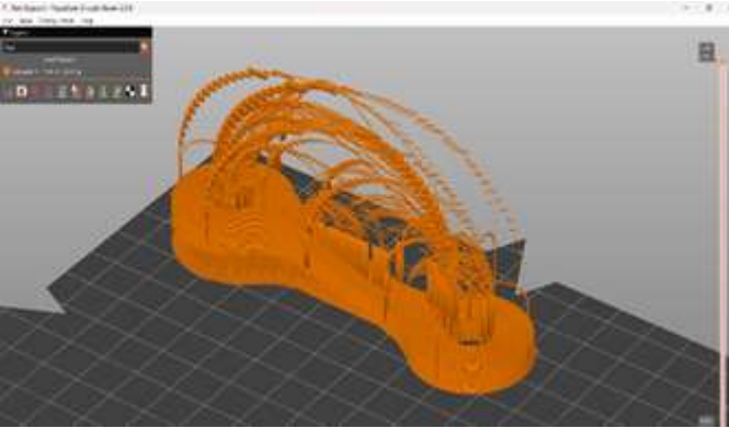
Fig. no:3.2 – Our final non planar toolpath in Prusa Slicer (Isometric view)
