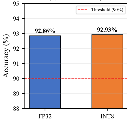
(b) Test Accuracy
