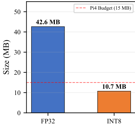
(a) Model Size
