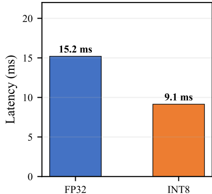
(c) Mean Inference Latency
