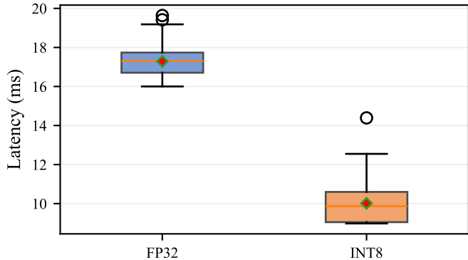
(a) Latency Distribution (n=200)
