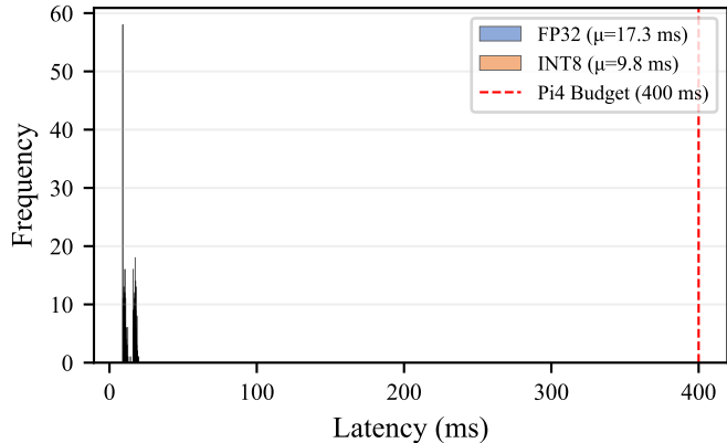
(b) Latency Histogram (n=200 runs)
