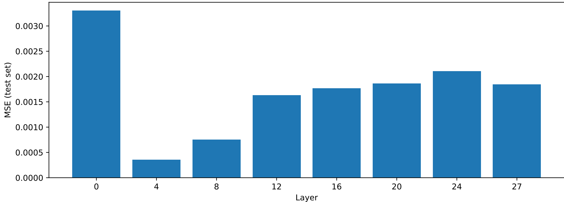
Belief State Regression MSE by Layer
