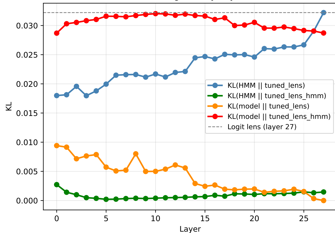
KL Divergence by Layer
