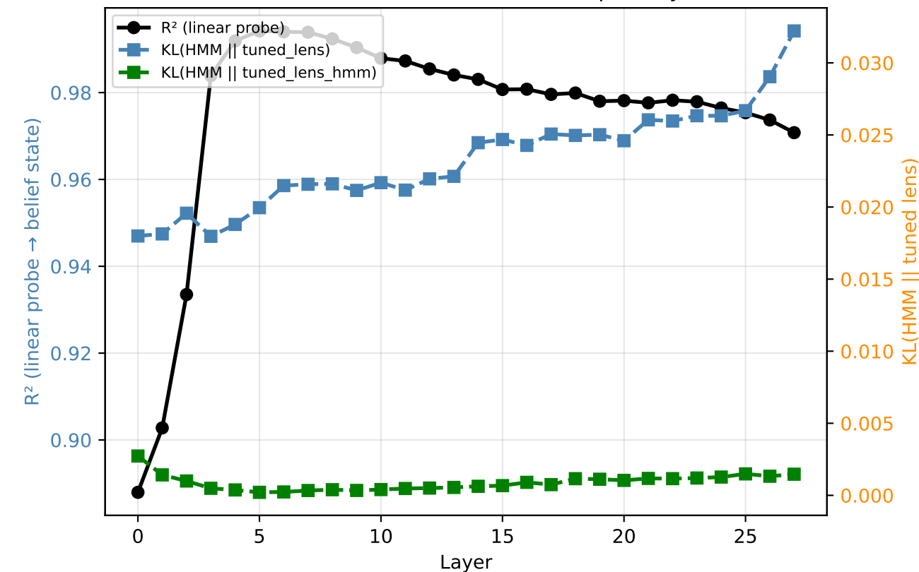
Belief-State R 2 vs Tuned-Lens KL per Layer
