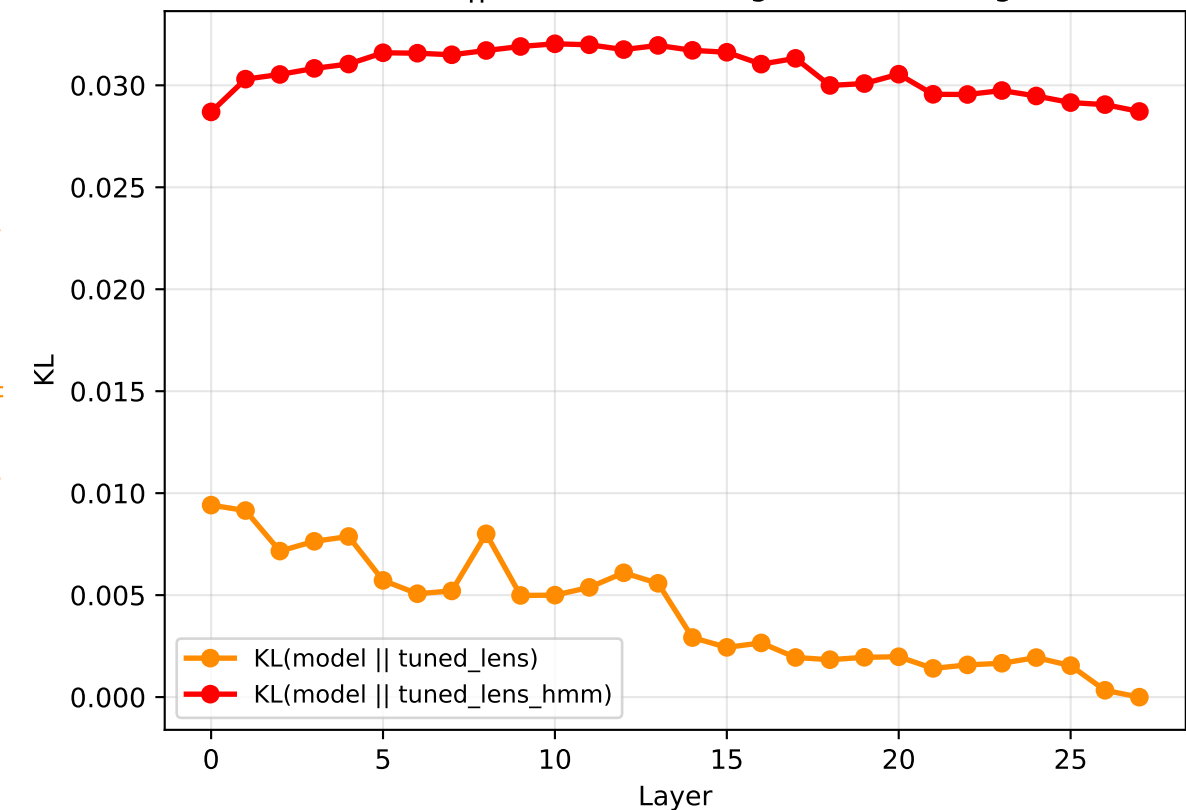
KL(model || lens): Model-target vs HMM-target
