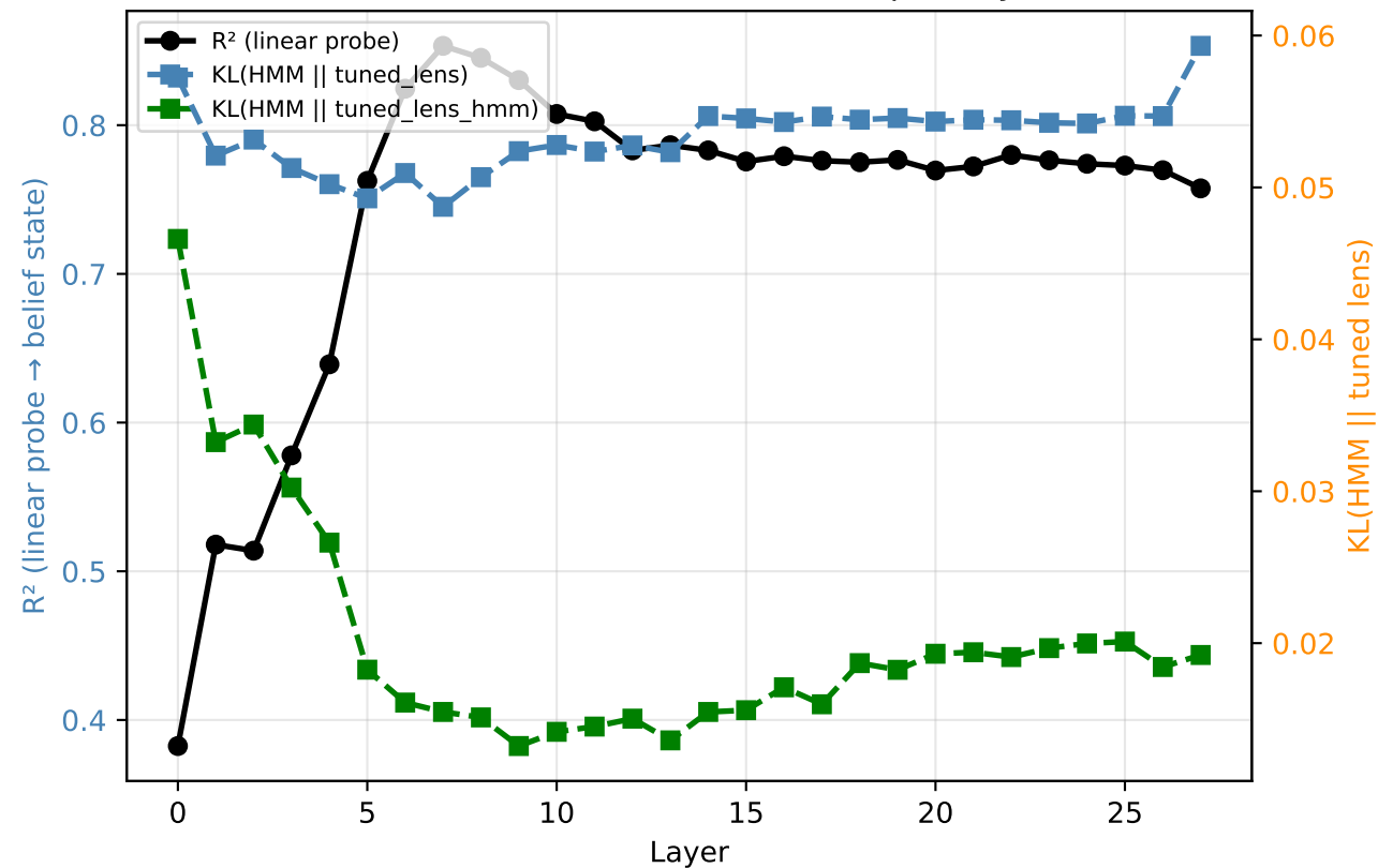
Belief-State R 2 vs Tuned-Lens KL per Layer
