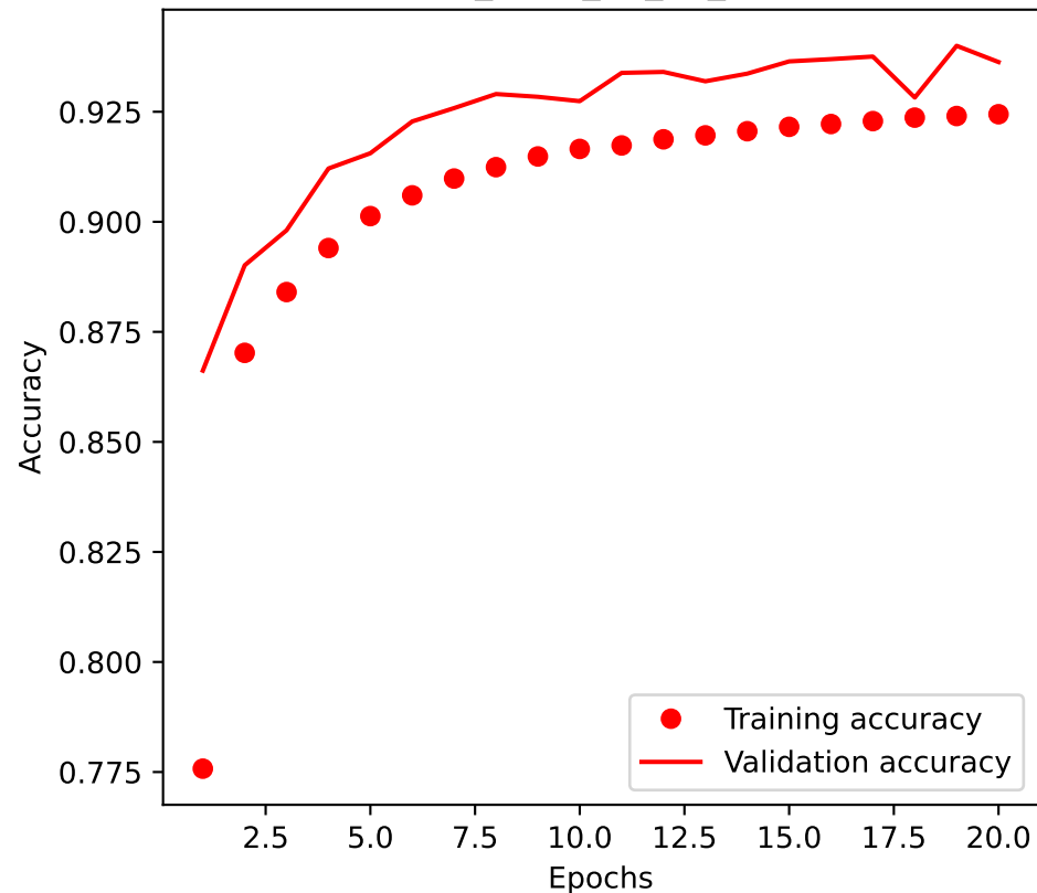
ITS2_2026_04_01_CNN
