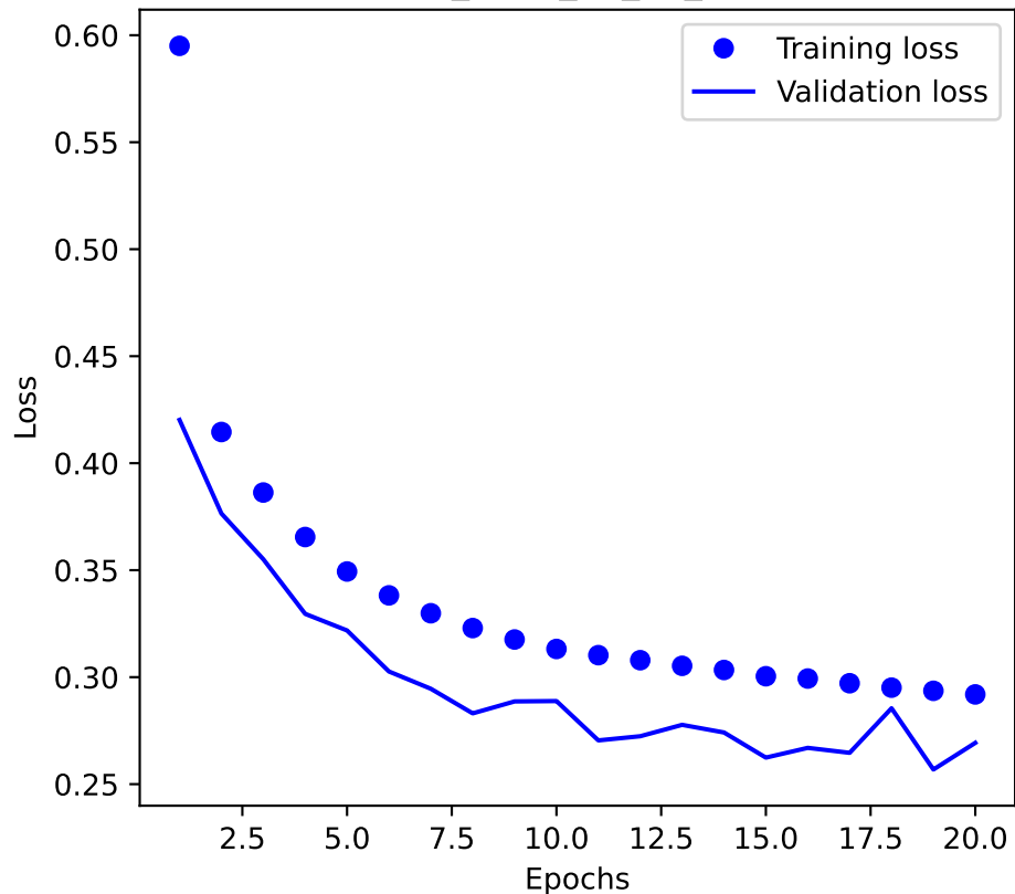
ITS2_2026_04_01_CNN
