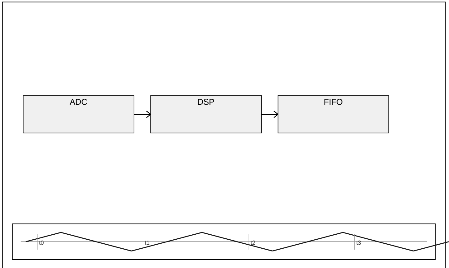
FIGURE 2-7. Page-wide datapath overview
