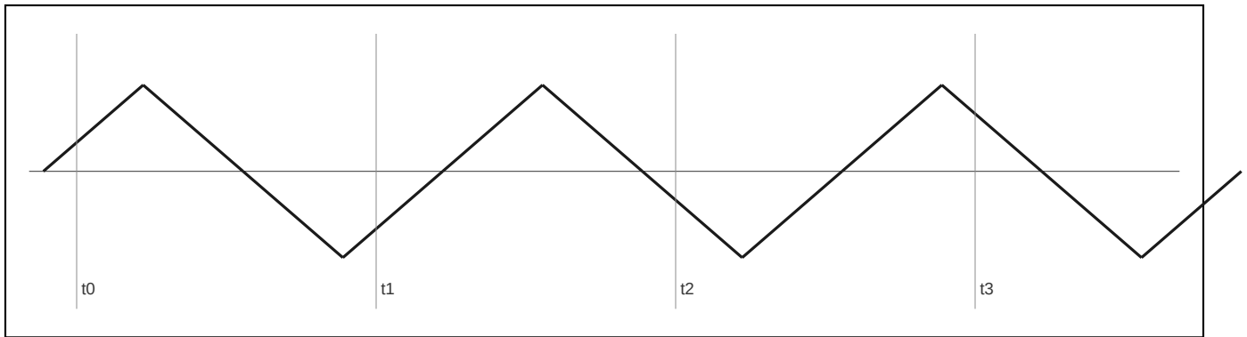
Figure 3-5. Sampled output
