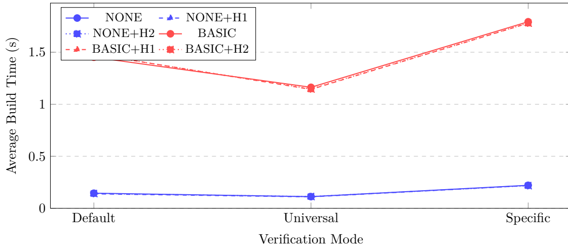
Figure 4: Average build time per configuration across verification modes. Blue lines = NONE family (no loop optimisation); red lines = BASIC family (with loop-collapse). Hints do not materially affect build time.
