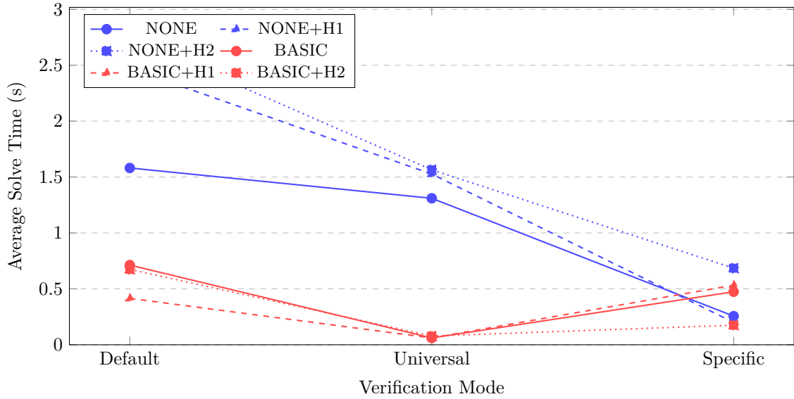
Figure 5: Average solve time per configuration (timeouts excluded from average). H2 ( heading_on_grid_always ) can raise solve time under NONE because the added assumption enlarges the CHC formula without the structural simplification that BASIC provides.
