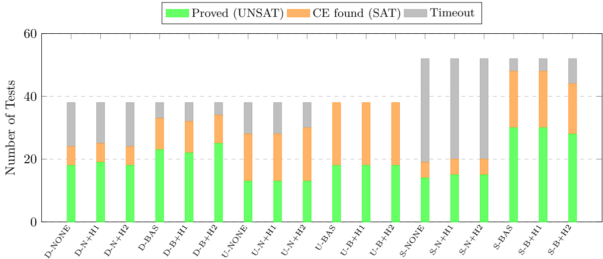
Figure 6: Verdict distribution across all modes (D=Default, U=Universal, S=Specific) and configurations (N=NONE, BAS=BASIC). Green = invariant proved; orange = expected counterexample found; gray = solver timed out.
