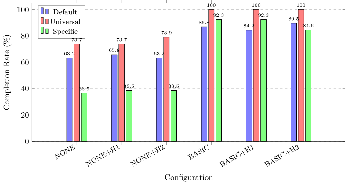
Figure 7: Completion rates broken down by verification mode. Universal mode reaches 100% under all BASIC variants. Specific mode is most sensitive to hint choice; H2 introduces regressions under BASIC.
