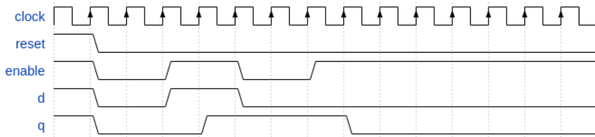
Figure 2: Timing Diagram
