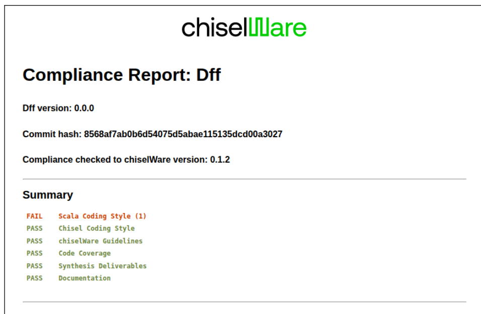
Figure 4.1: ADR compliance report summary showing pass/fail status for each of the six rule categories.
