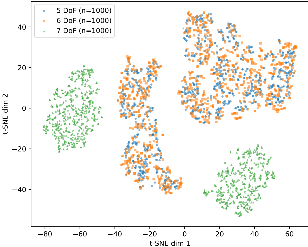
Penultimate-layer features of the shared meta-kinematics model
