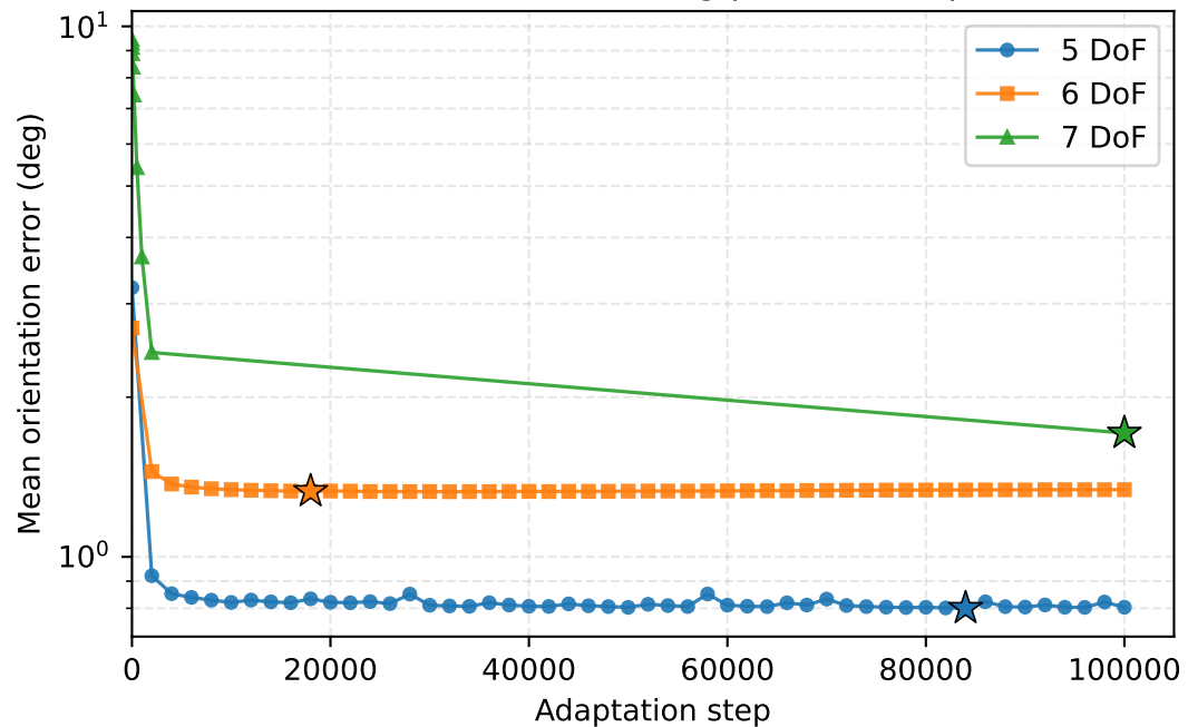
(b) Orientation error during per-DoF adaptation
