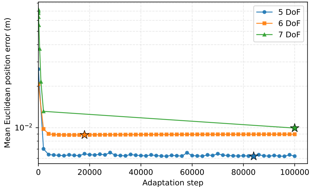
(a) Position error during per-DoF adaptation
