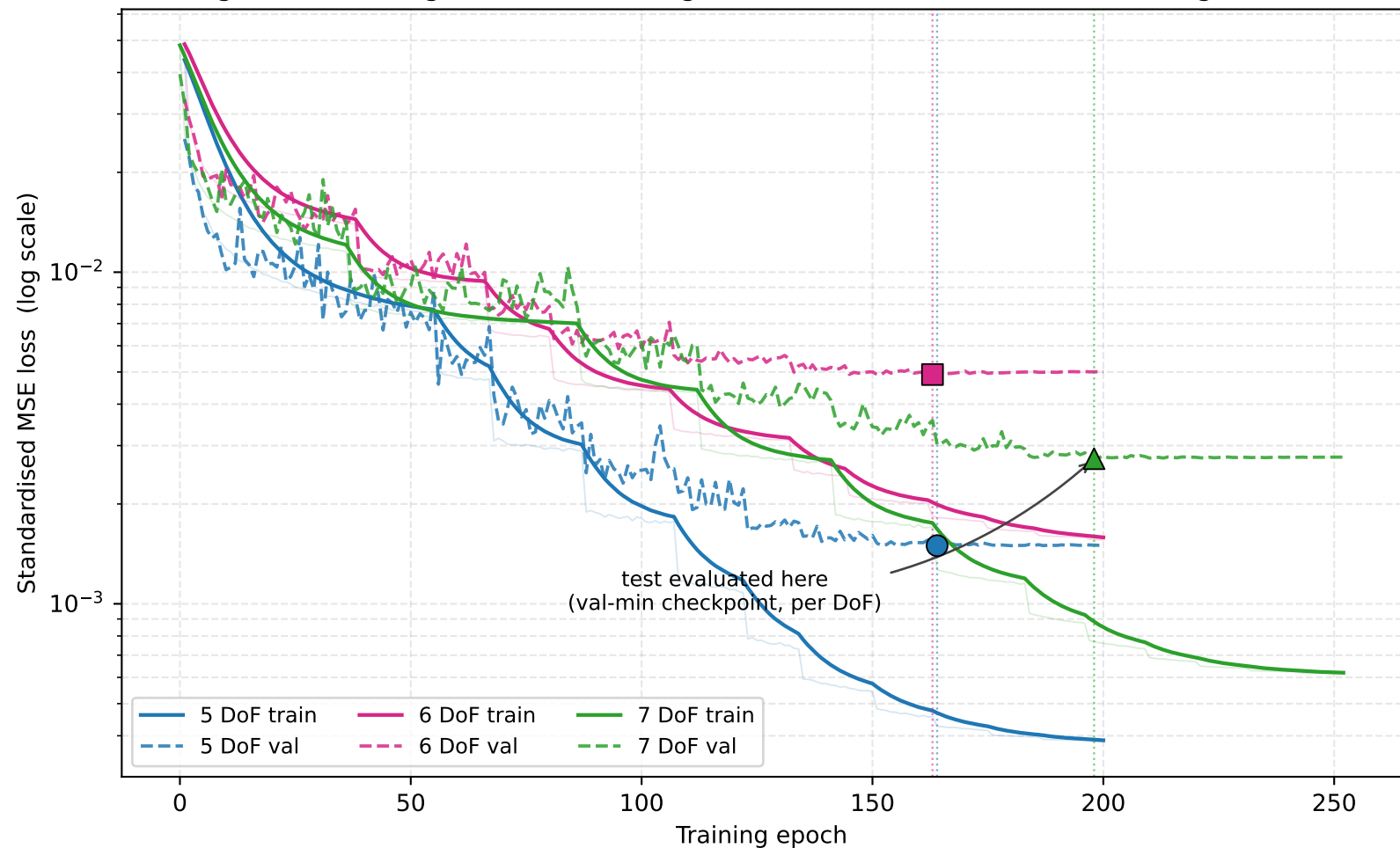
Figure 5.1 — Single-task FK training curves for the 5, 6 and 7 DoF configurations
