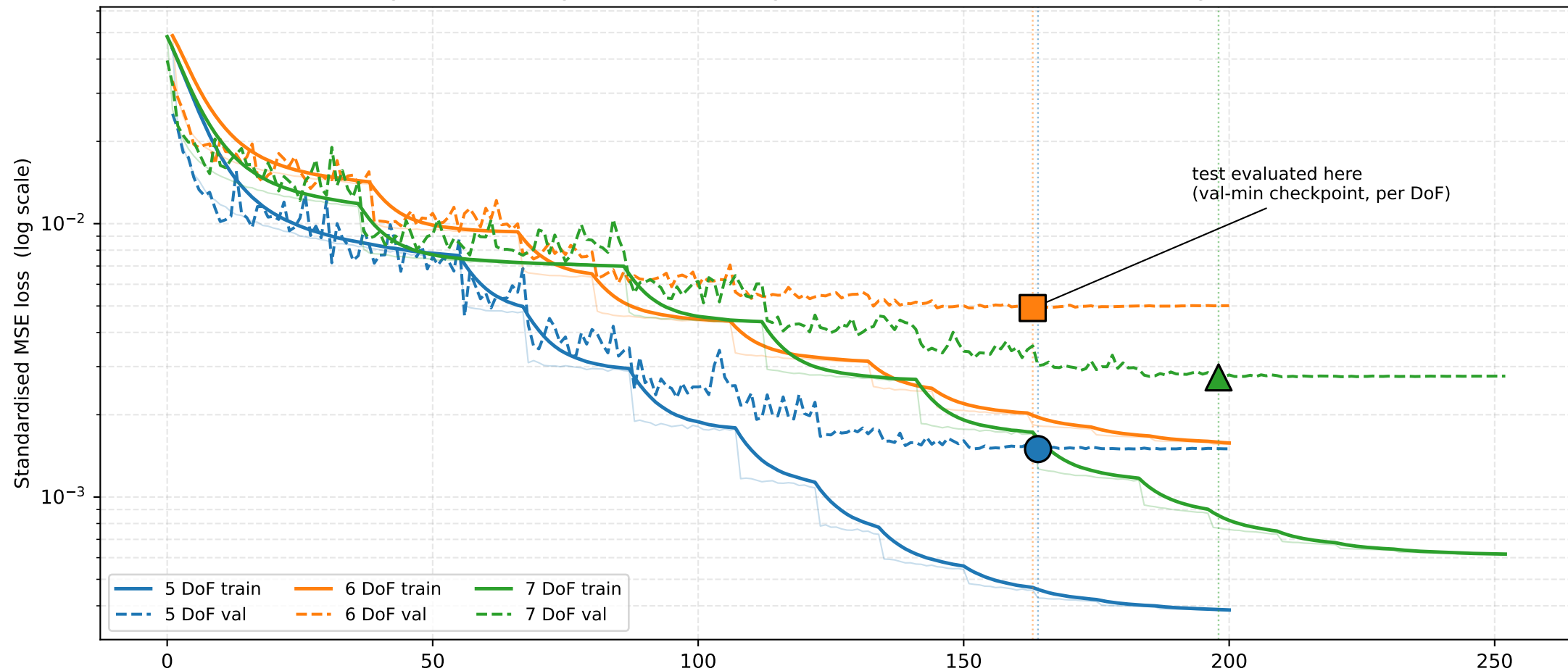
Figure 5.1 — Single-task FK training curves for the 5, 6 and 7 DoF configurations
