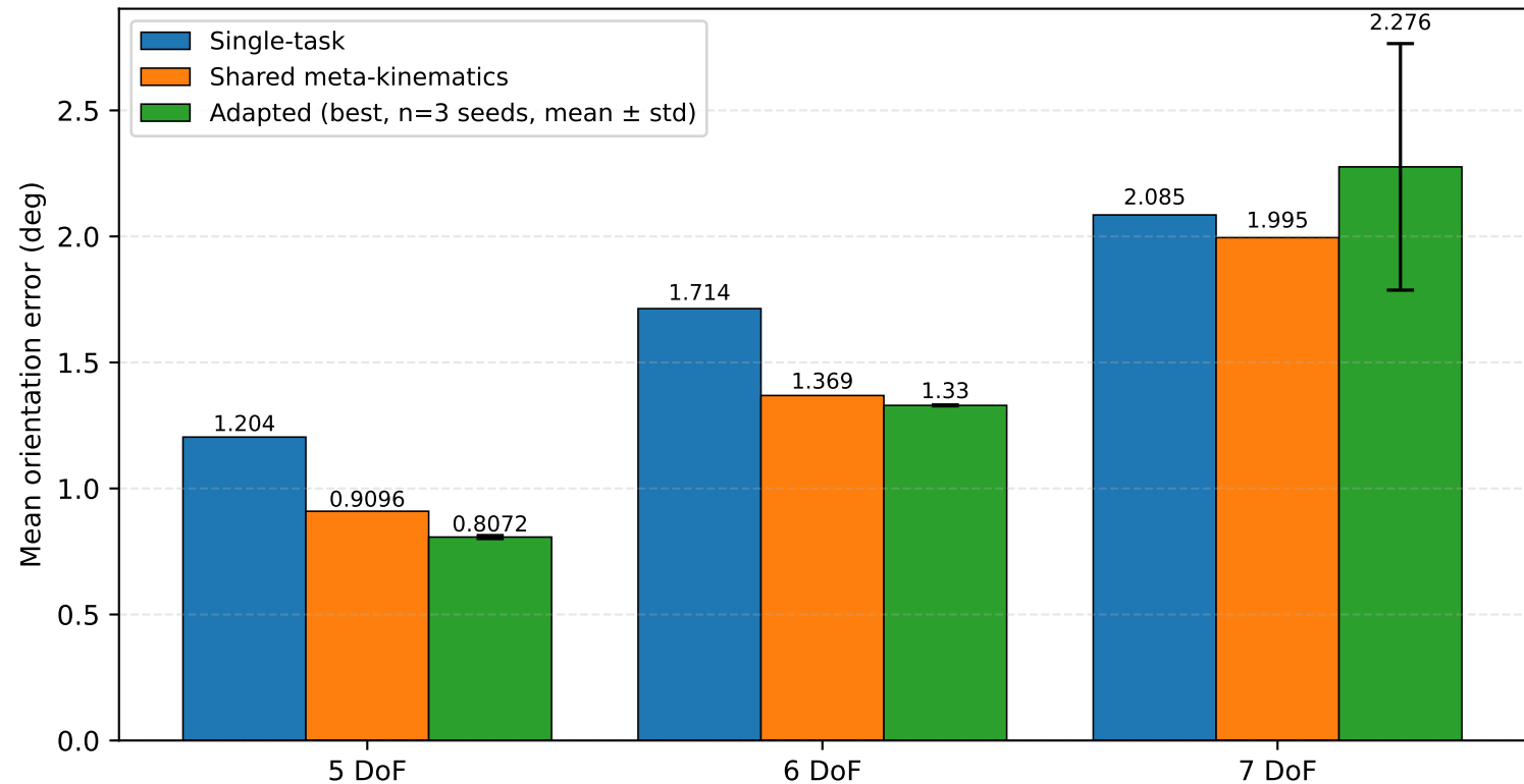
Figure 5.4 — Orientation error per DoF configuration
