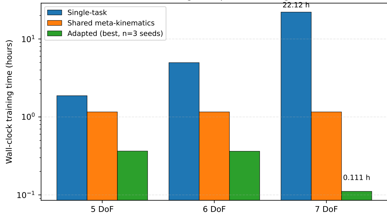
Wall-clock training time per DoF configuration
