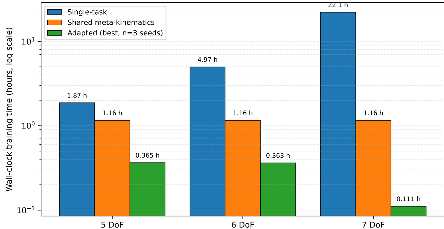
Figure 5.5 — Wall-clock training time per DoF configuration
