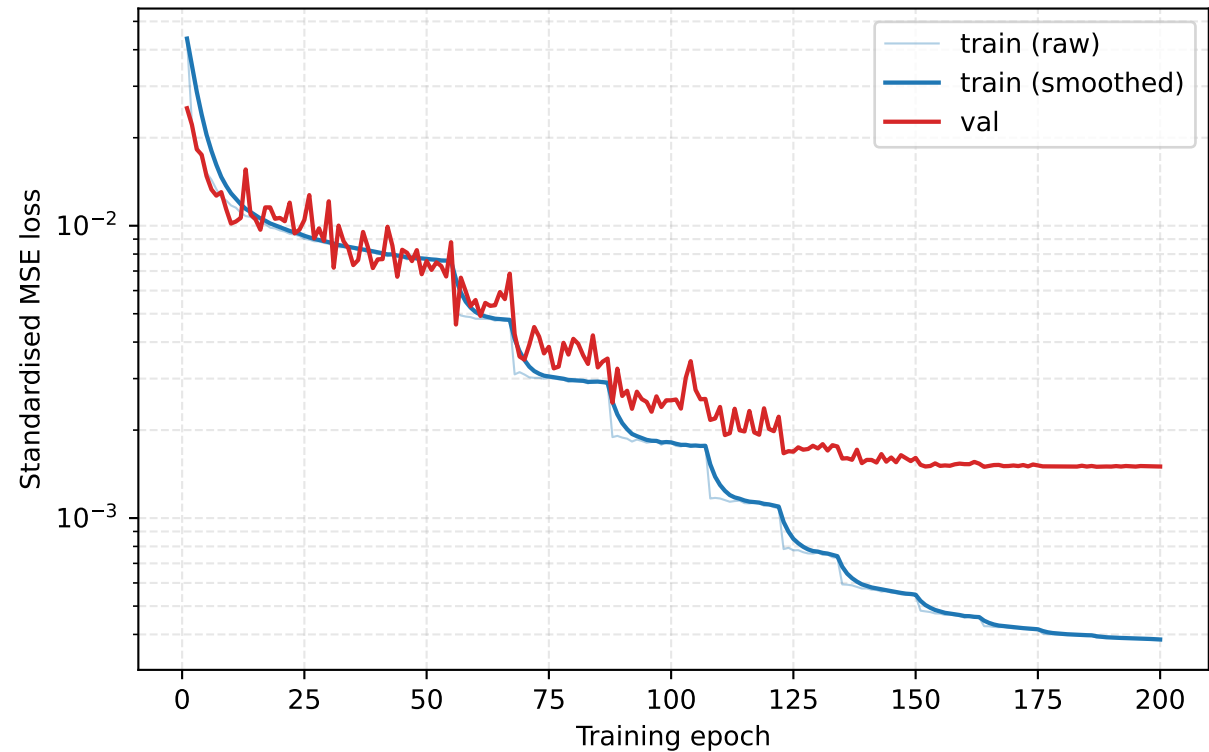
Stage 1 — Single-task 5-DoF FK training
