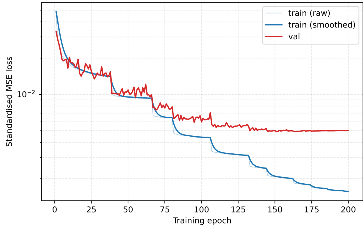
Stage 1 — Single-task 6-DoF FK training
