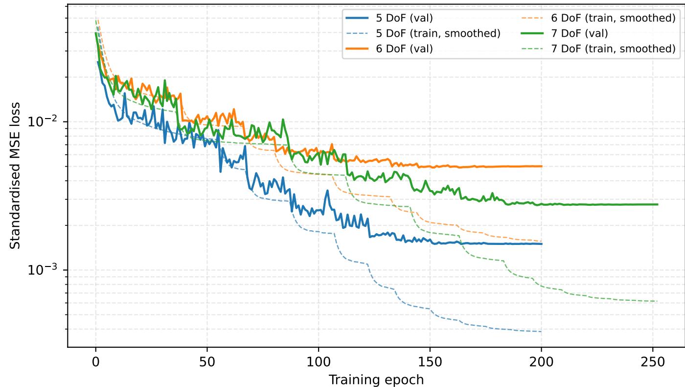
Stage 1 — Single-task FK training across DoF configurations
