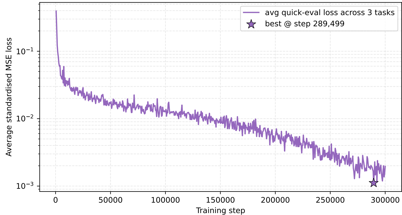
Stage 2 — Quick-eval loss used for best-checkpoint selection
