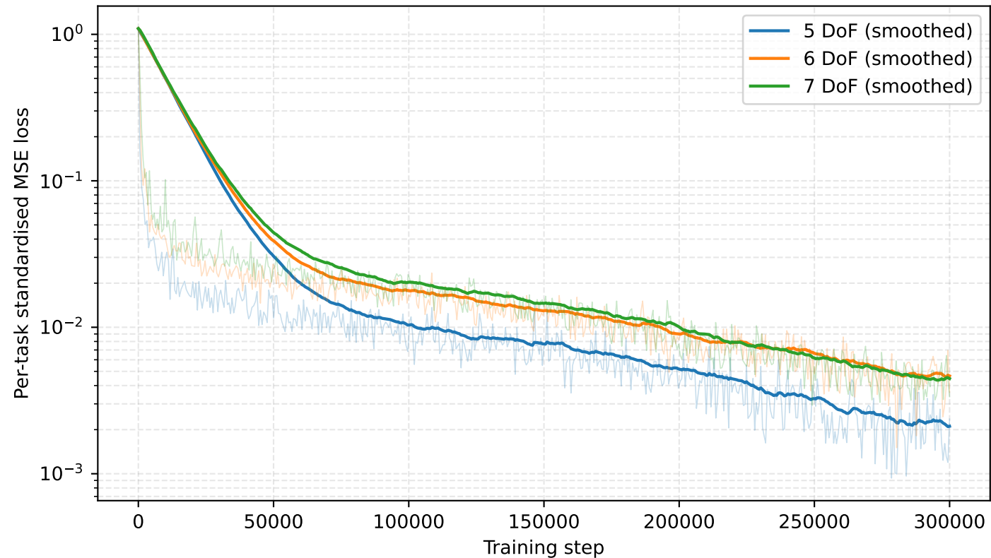
Stage 2 — Shared meta-kinematics training (seed=42, 300 000 steps)
