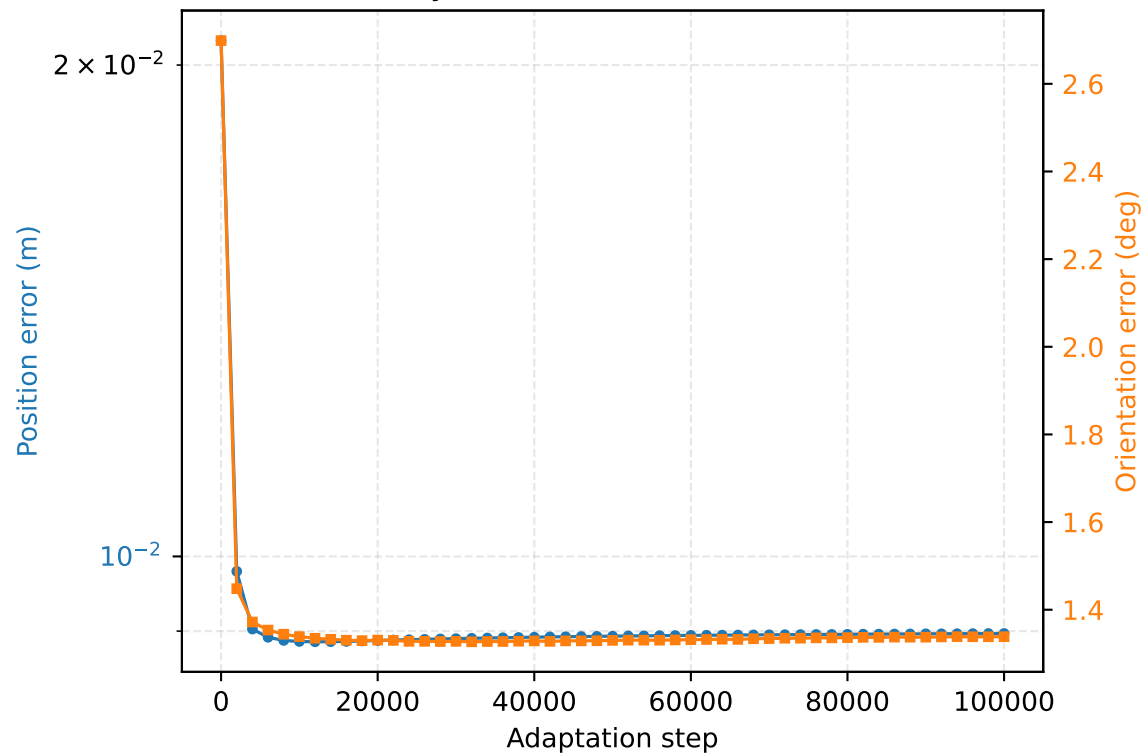
(b) Query-set held-out metrics — 6 DoF
