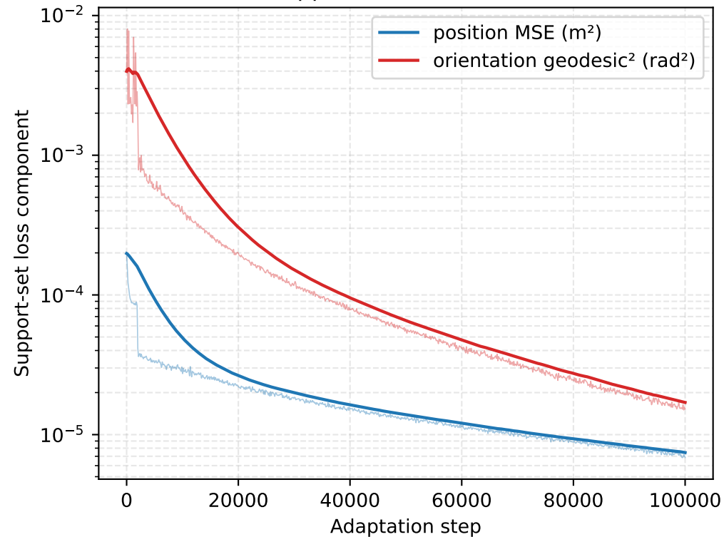
(a) Support-set losses — 6 DoF
