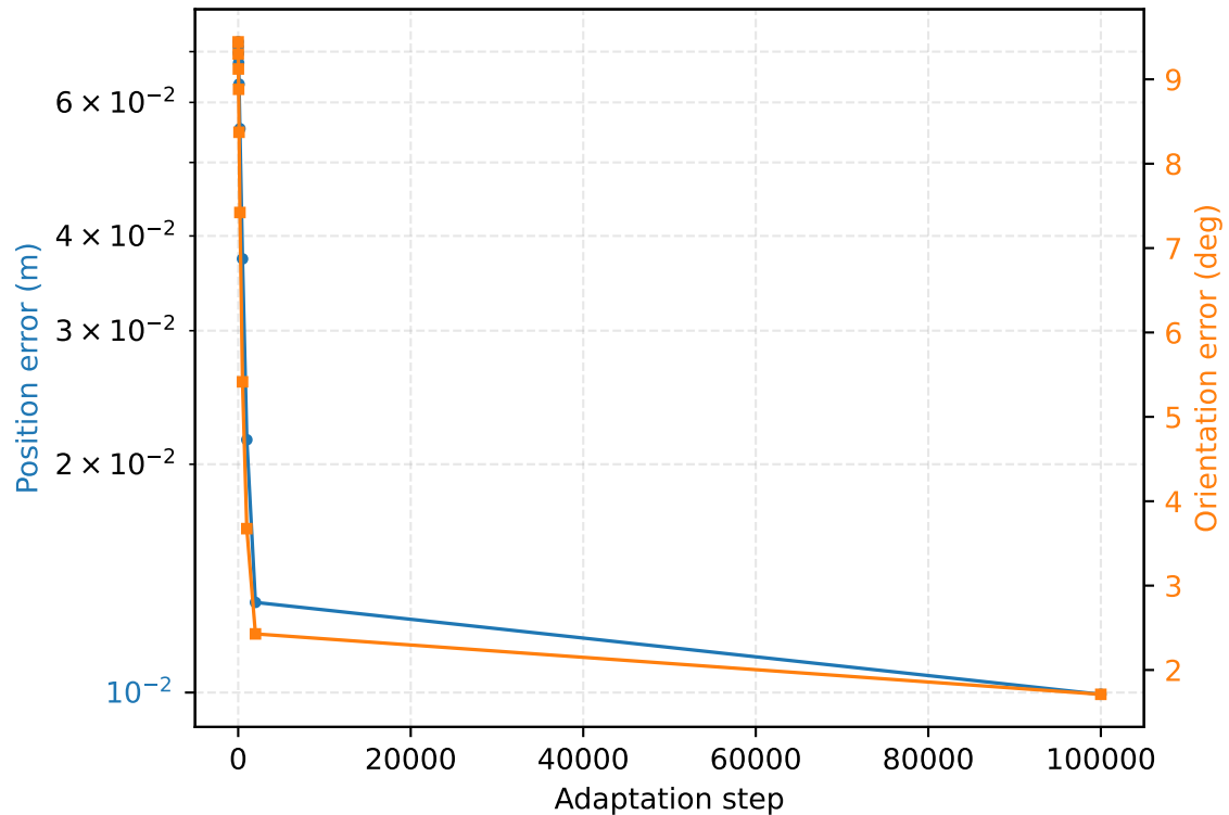
(b) Query-set held-out metrics — 7 DoF
