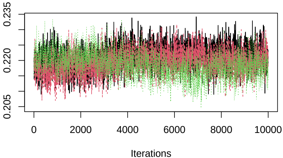
Trace of sigmas_1
