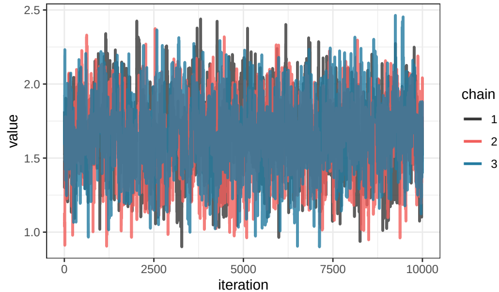
Traceplot of value(log_PLASMA_NFL)
