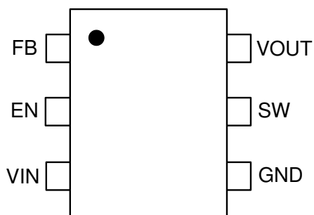
Figure 5-1. DRL Package 6-Pin SOT563 Top View
