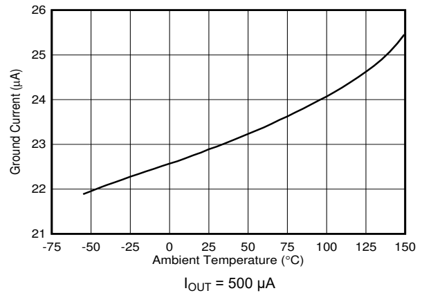
Figure 5-26. Ground Current
