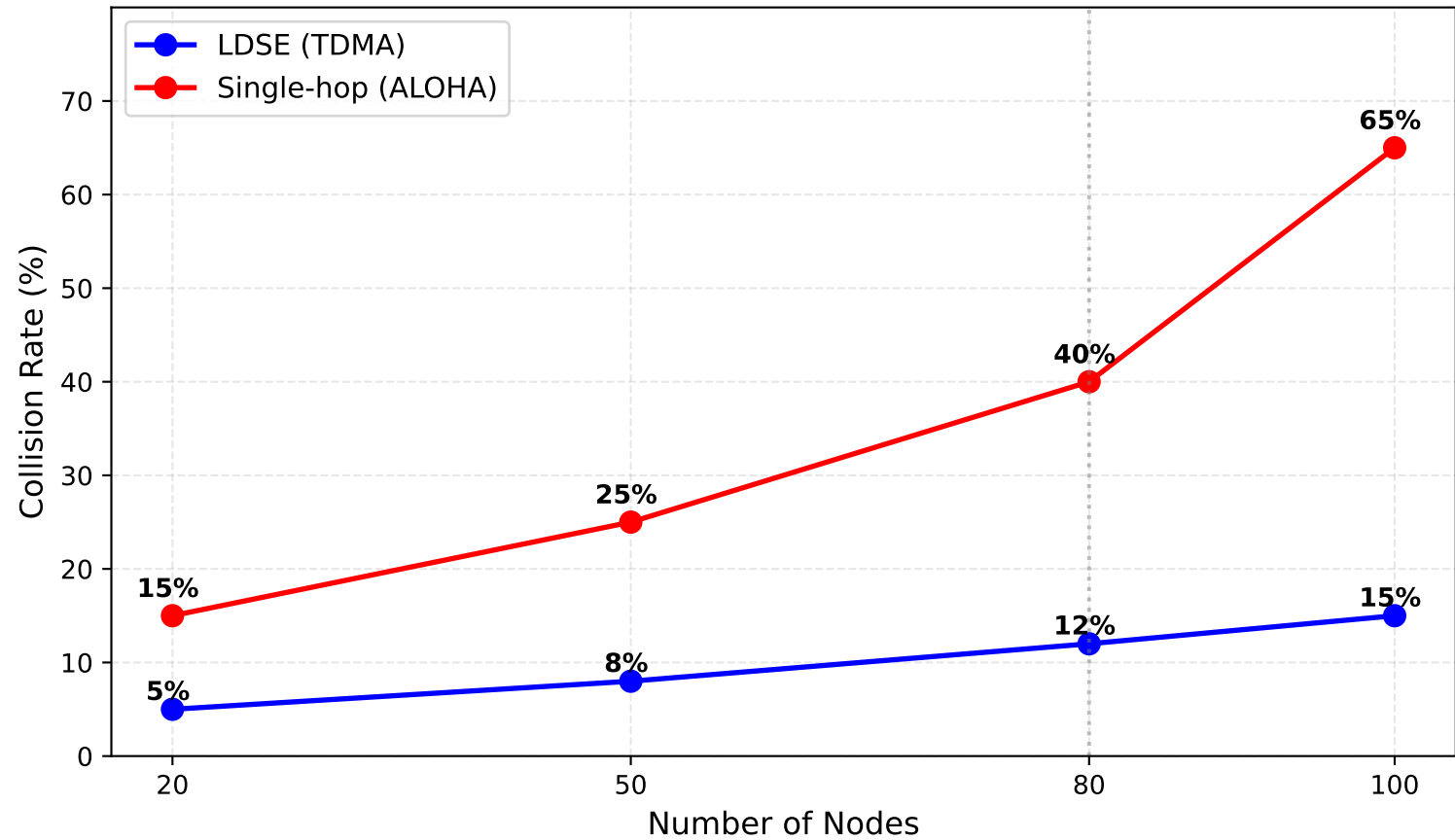
Packet Collision Rate vs. Number of Nodes
