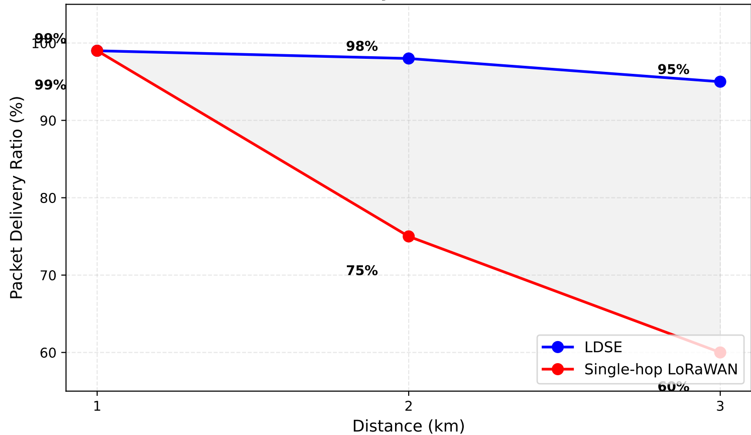
Packet Delivery Ratio vs. Distance
