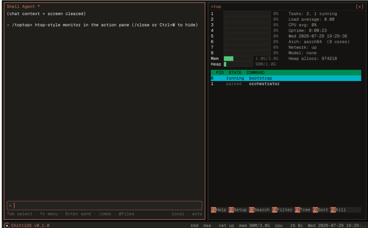
Figure 2: ChittiOS running, captured from the guest’s own framebuffer through the QEMU monitor ( screendump ) rather than reconstructed from a terminal transcript. The chat pane on the left is the shell agent — the orchestrator whose authority §3.3 describes — and the right pane is a live /top , showing the eight cores the SMP fleet is running on, the two tasks alive at that moment (the bootstrap task and the parked capability-owning orchestrator), and the kernel heap. Everything in the figure is one process image on bare metal: compositor, scheduler, network stack, and the inference engine that would occupy the “Model” slot on a model-loaded boot.
